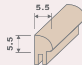
TOP & BOTTOM STRIP
