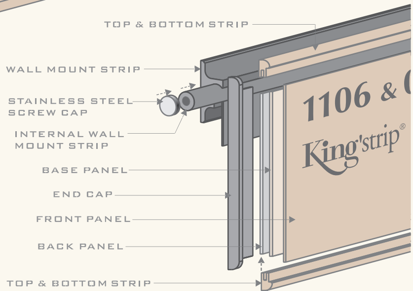
EXPLODED VIEW
