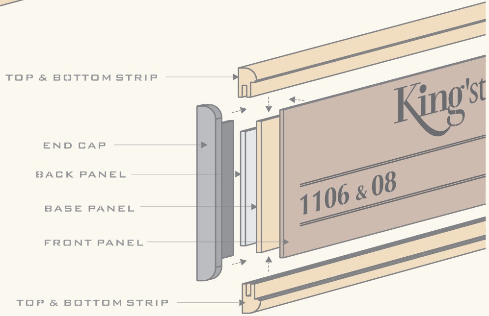
EXPLODED VIEW
