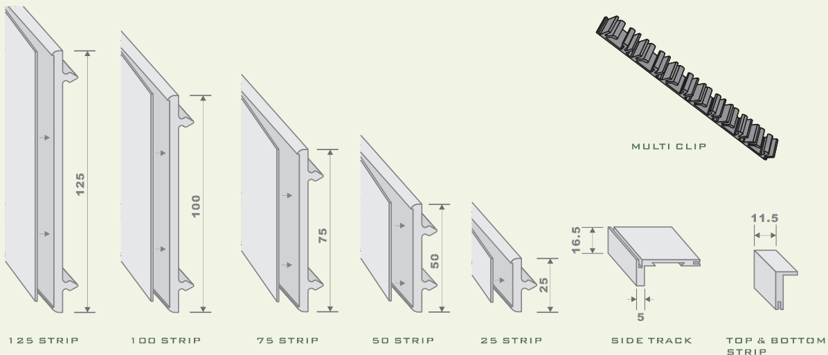
EXPLODED VIEW
