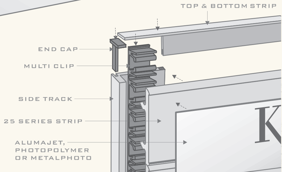
EXPLODED VIEW
