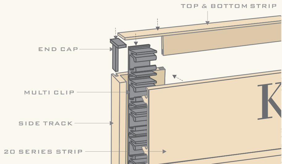
EXPLODED VIEW
